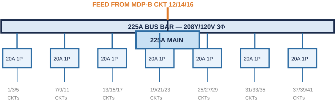
Figure 3 — Panel LP-5A One-Line Wiring Diagram (Schematic — Not to Scale)
